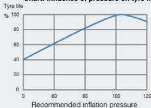
Chart: Influence of pressure on tyre life
